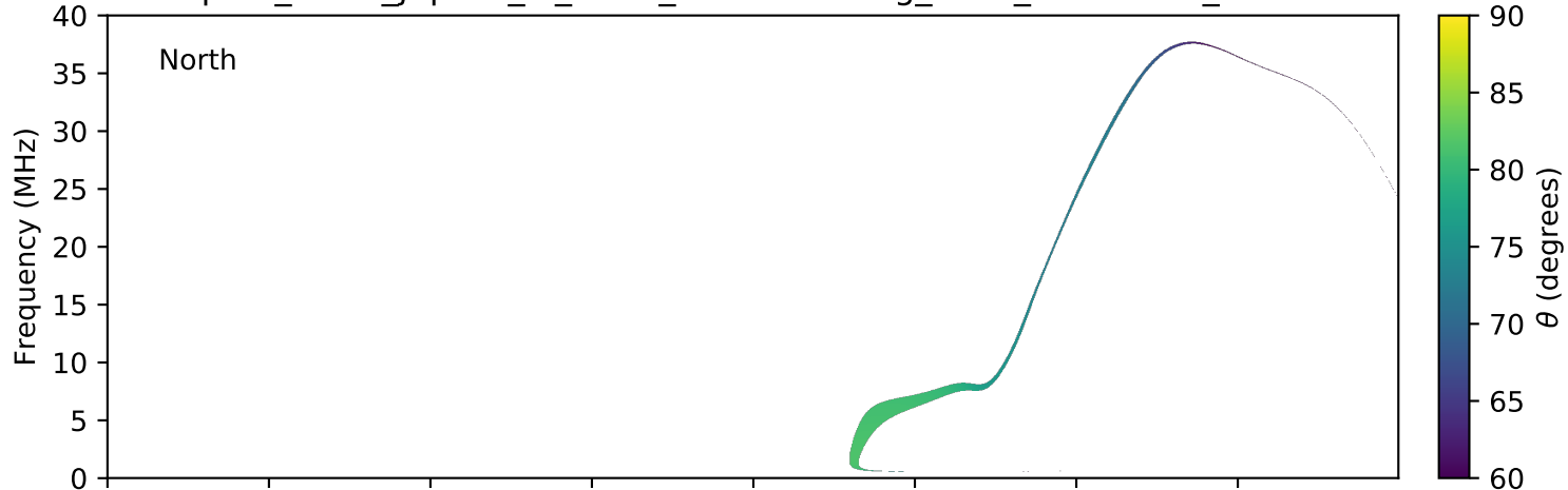
expres_earth_jupiter_io_isaac_lossc-wid1deg_5kev_20160206_v01.cdf
