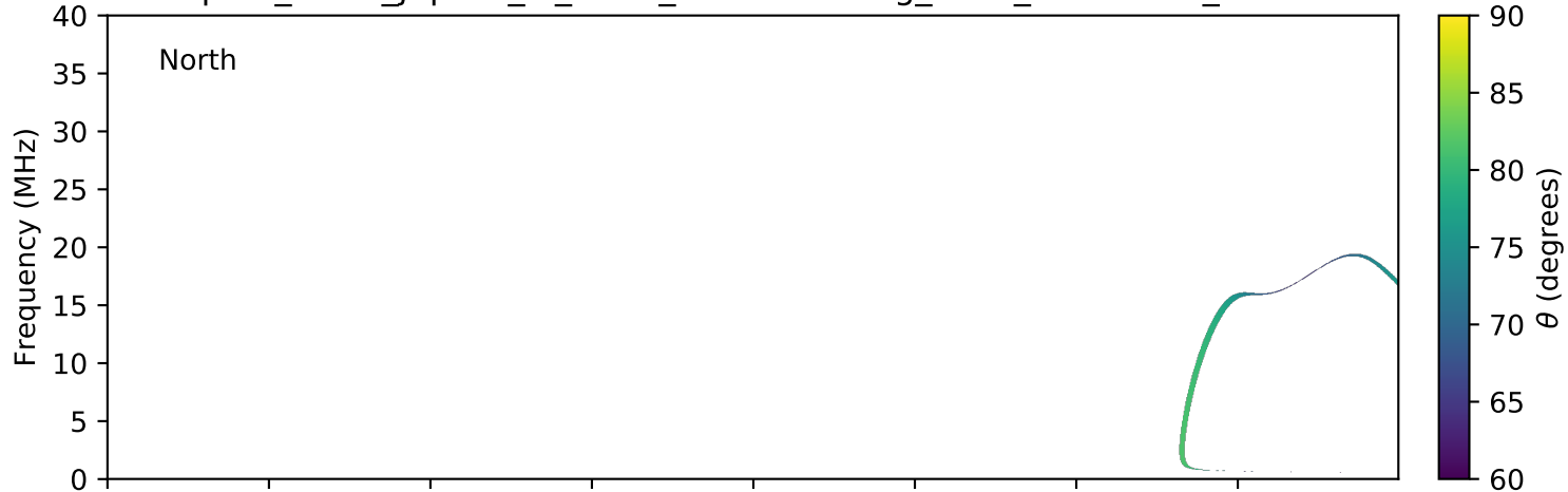
expres_earth_jupiter_io_isaac_lossc-wid1deg_5kev_20160204_v01.cdf
