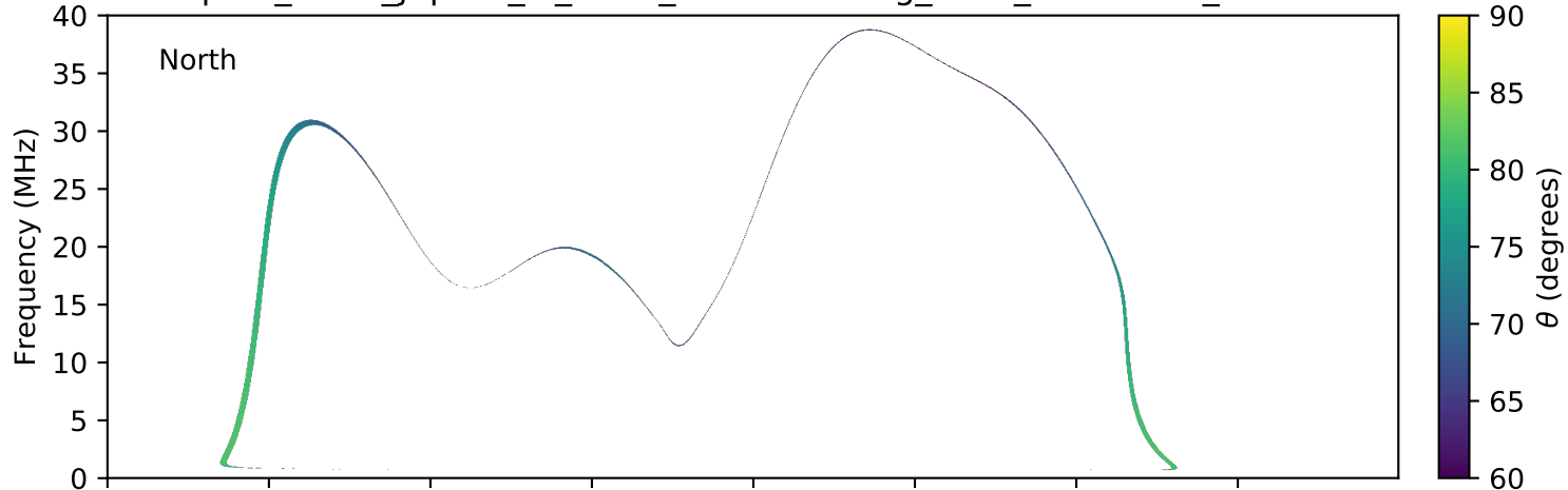
expres_earth_jupiter_io_isaac_lossc-wid1deg_5kev_20160203_v01.cdf
