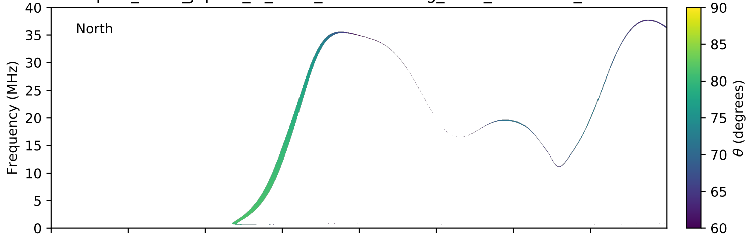
expres_earth_jupiter_io_isaac_lossc-wid1deg_5kev_20160201_v01.cdf
