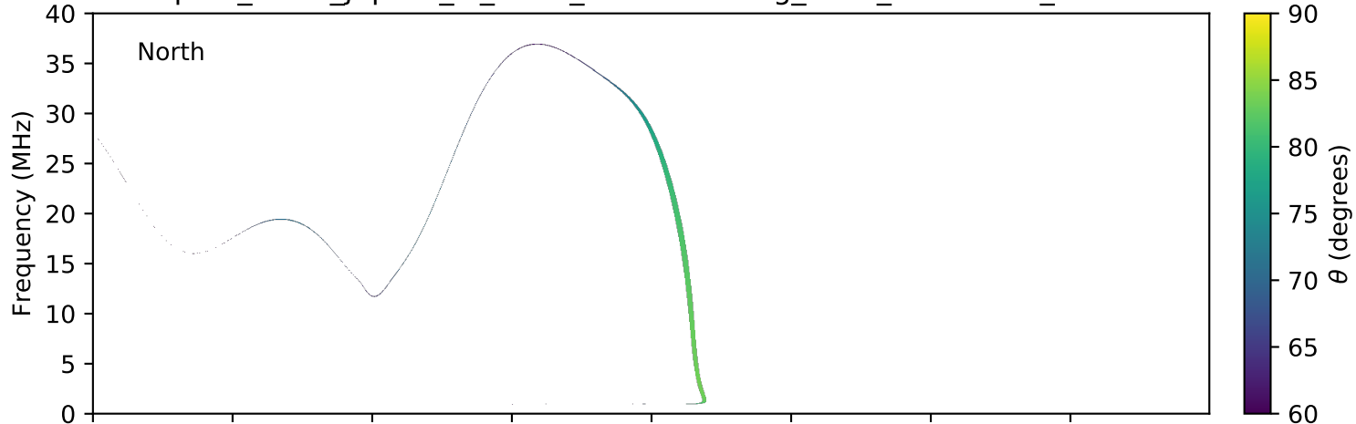
expres_earth_jupiter_io_isaac_lossc-wid1deg_3kev_20160221_v01.cdf
