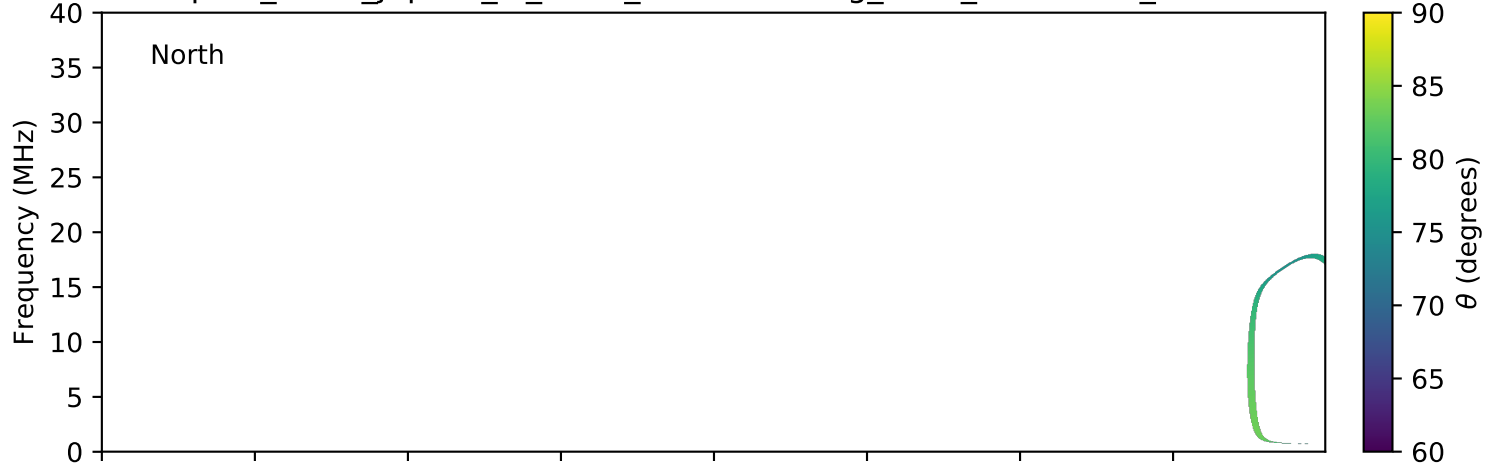
expres_earth_jupiter_io_isaac_lossc-wid1deg_3kev_20160218_v01.cdf
