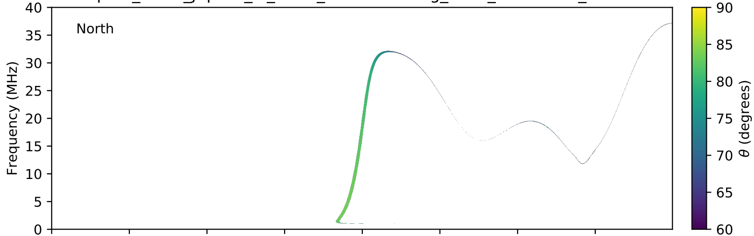
expres_earth_jupiter_io_isaac_lossc-wid1deg_3kev_20160215_v01.cdf
