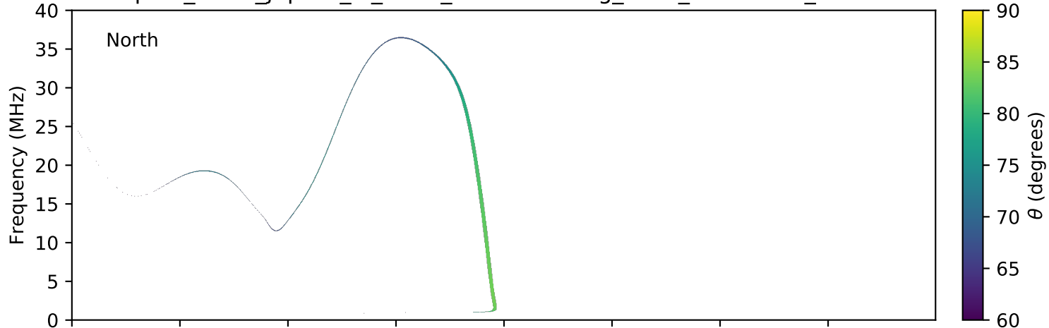
expres_earth_jupiter_io_isaac_lossc-wid1deg_3kev_20160214_v01.cdf
