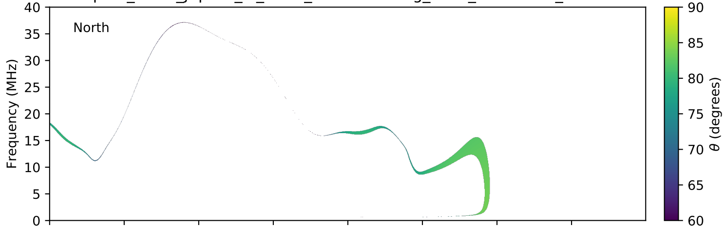
expres_earth_jupiter_io_isaac_lossc-wid1deg_3kev_20160212_v01.cdf
