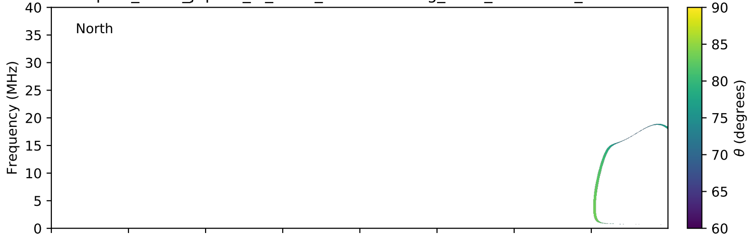
expres_earth_jupiter_io_isaac_lossc-wid1deg_3kev_20160211_v01.cdf
