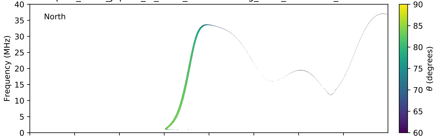
expres_earth_jupiter_io_isaac_lossc-wid1deg_3kev_20160208_v01.cdf
