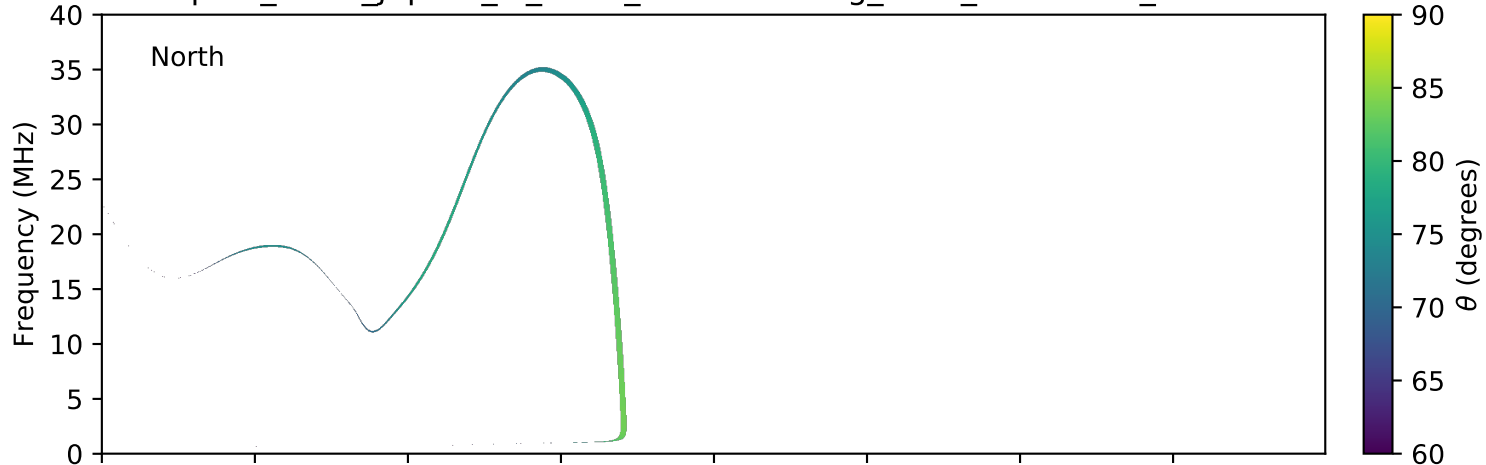
expres_earth_jupiter_io_isaac_lossc-wid1deg_3kev_20160207_v01.cdf
