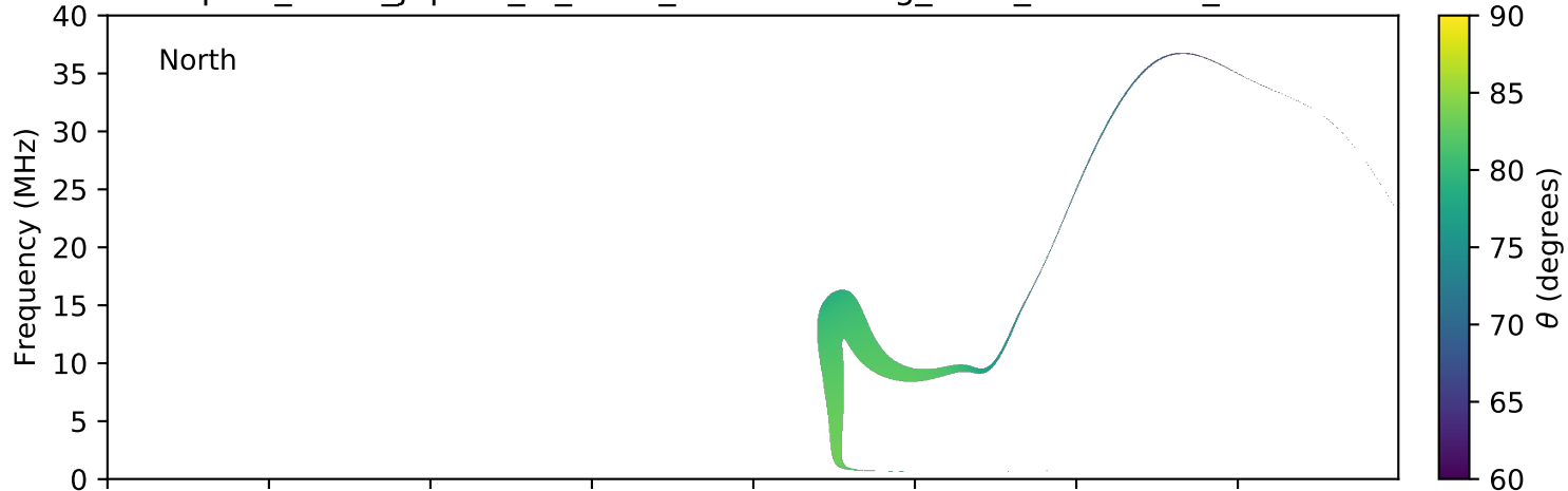
expres_earth_jupiter_io_isaac_lossc-wid1deg_3kev_20160206_v01.cdf
