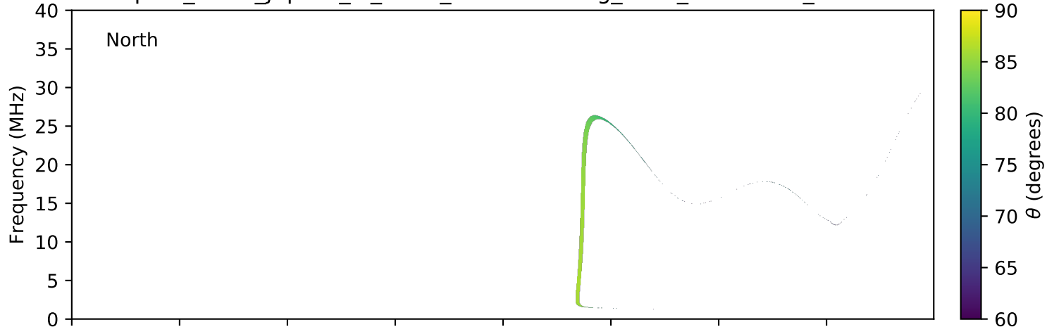
expres_earth_jupiter_io_isaac_lossc-wid1deg_1kev_20160229_v01.cdf
