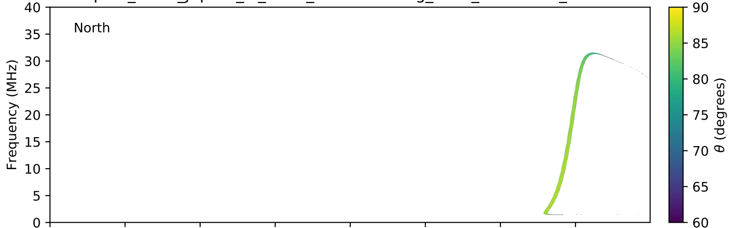
expres_earth_jupiter_io_isaac_lossc-wid1deg_1kev_20160227_v01.cdf
