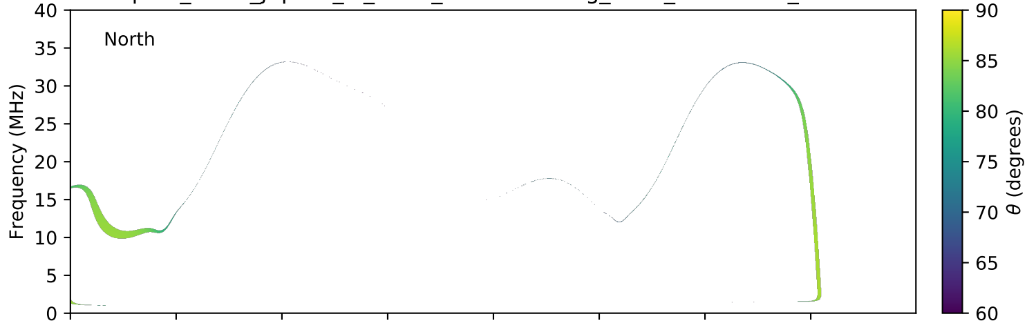
expres_earth_jupiter_io_isaac_lossc-wid1deg_1kev_20160226_v01.cdf
