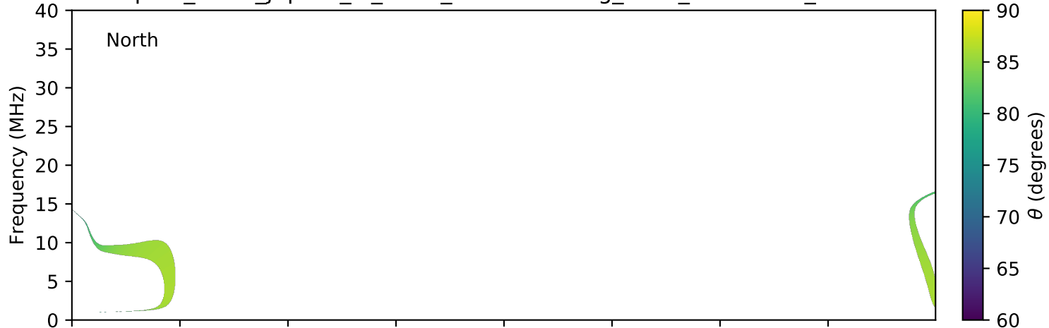
expres_earth_jupiter_io_isaac_lossc-wid1deg_1kev_20160225_v01.cdf
