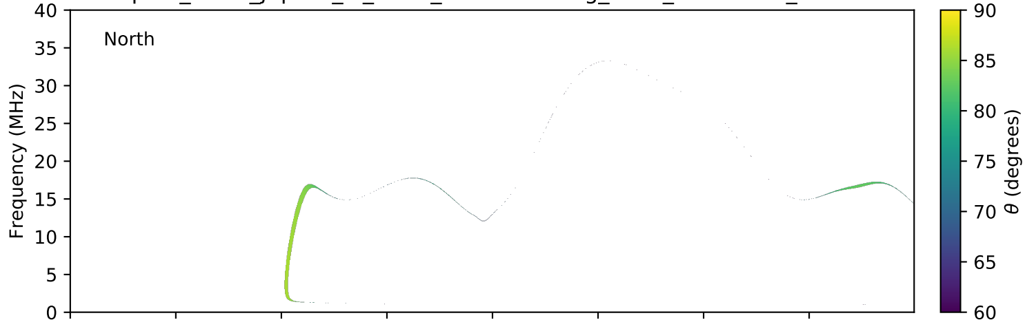
expres_earth_jupiter_io_isaac_lossc-wid1deg_1kev_20160224_v01.cdf
