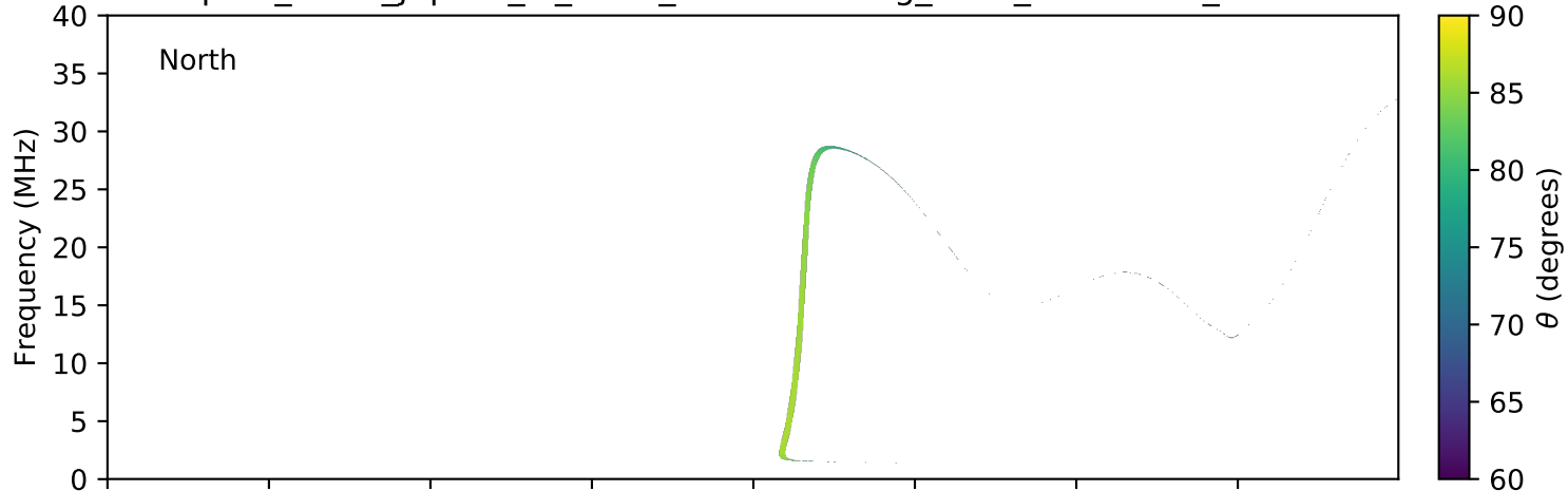
expres_earth_jupiter_io_isaac_lossc-wid1deg_1kev_20160222_v01.cdf
