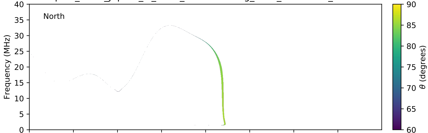
expres_earth_jupiter_io_isaac_lossc-wid1deg_1kev_20160221_v01.cdf
