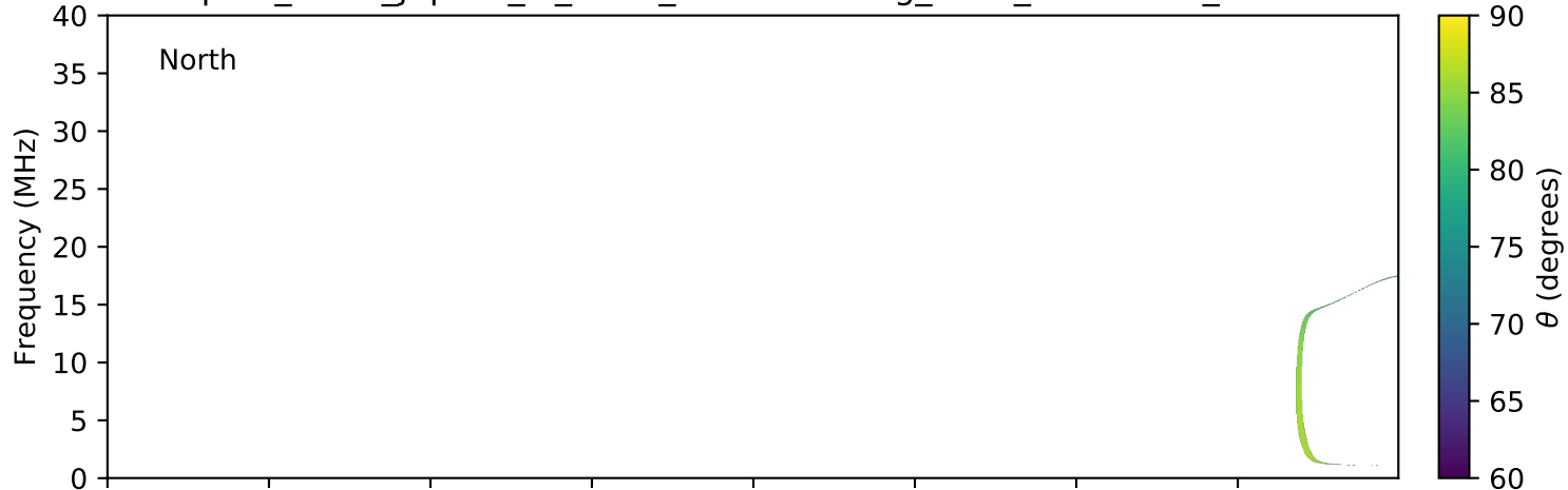
expres_earth_jupiter_io_isaac_lossc-wid1deg_1kev_20160218_v01.cdf
