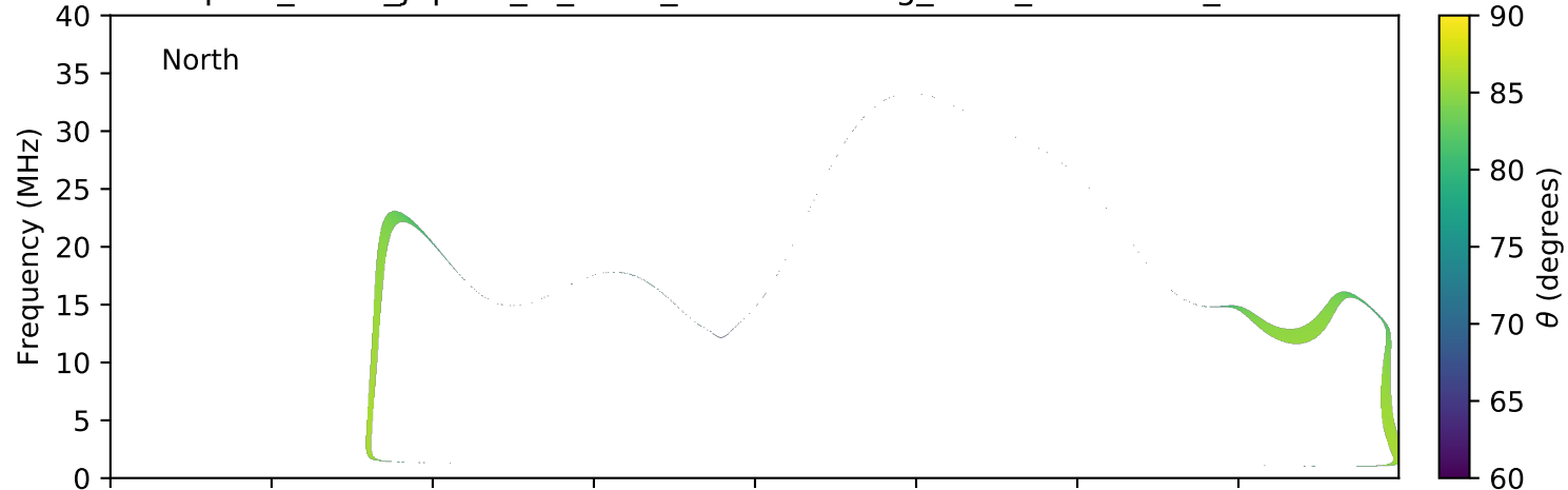
expres_earth_jupiter_io_isaac_lossc-wid1deg_1kev_20160217_v01.cdf
