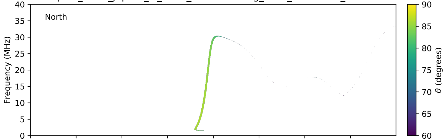
expres_earth_jupiter_io_isaac_lossc-wid1deg_1kev_20160215_v01.cdf
