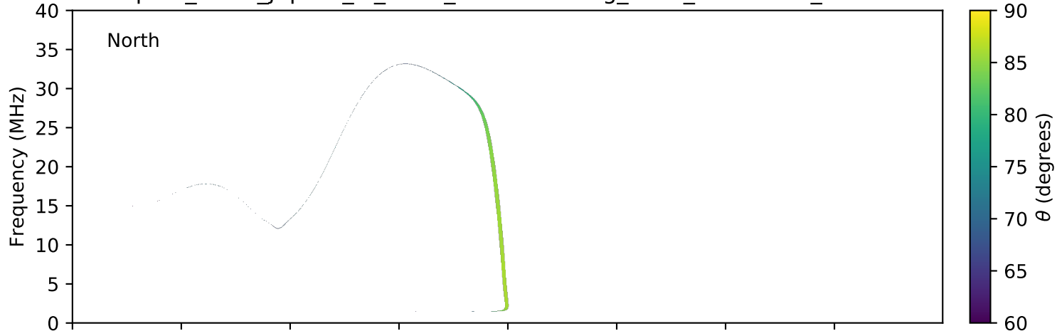
expres_earth_jupiter_io_isaac_lossc-wid1deg_1kev_20160214_v01.cdf
