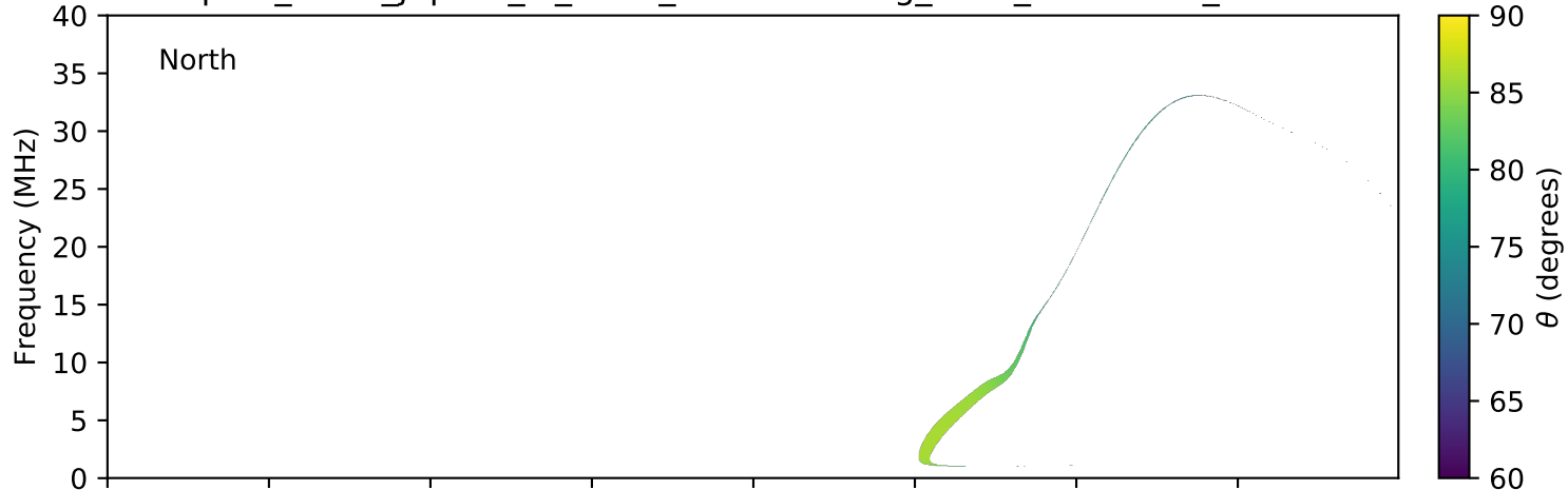
expres_earth_jupiter_io_isaac_lossc-wid1deg_1kev_20160213_v01.cdf
