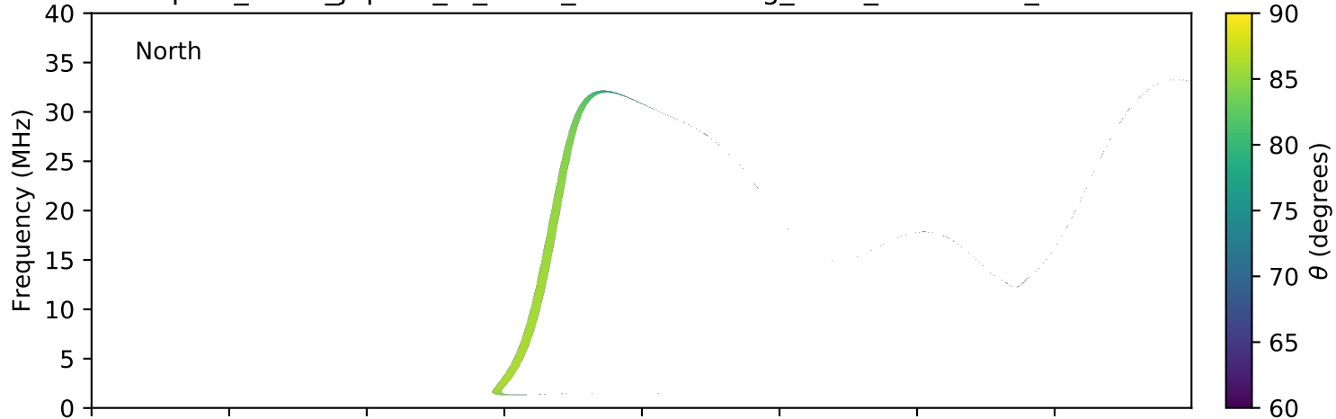
expres_earth_jupiter_io_isaac_lossc-wid1deg_1kev_20160208_v01.cdf
