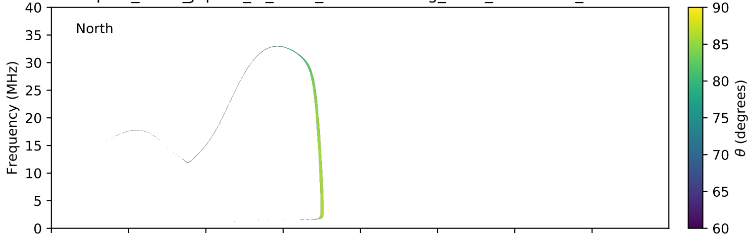
expres_earth_jupiter_io_isaac_lossc-wid1deg_1kev_20160207_v01.cdf
