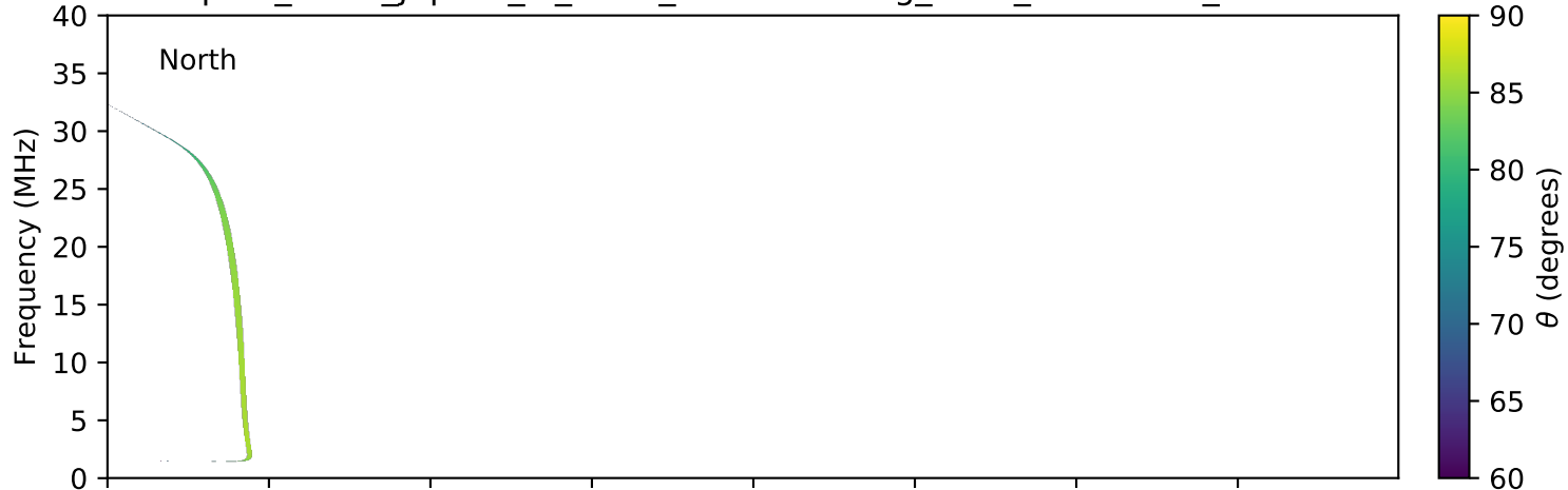
expres_earth_jupiter_io_isaac_lossc-wid1deg_1kev_20160202_v01.cdf
