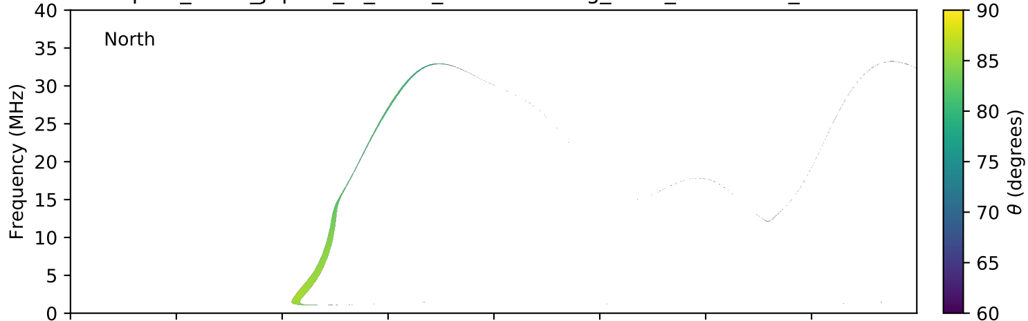
expres_earth_jupiter_io_isaac_lossc-wid1deg_1kev_20160201_v01.cdf
