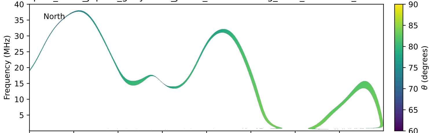
expres_earth_jupiter_ganymede_jrm33_lossc-wid1deg_3kev_20160218_v11.cdf
