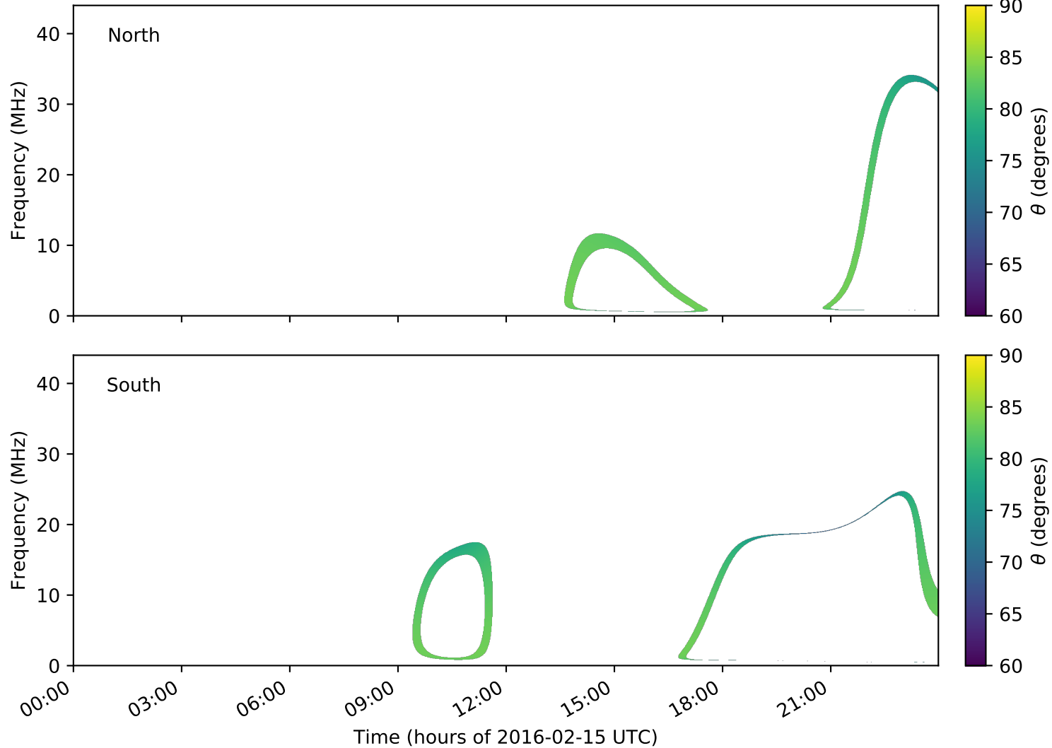
expres_earth_jupiter_ganymede_jrm09_lossc-wid1deg_3kev_20160215_v01.cdf
