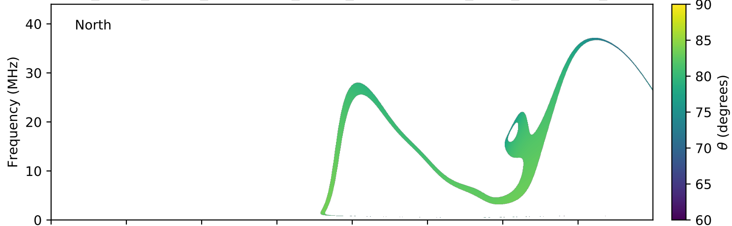
expres_earth_jupiter_ganymede_jrm09_lossc-wid1deg_3kev_20160201_v01.cdf
