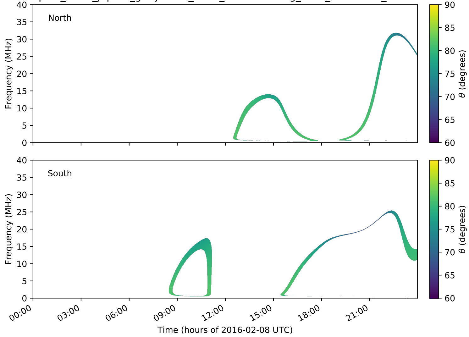
expres_earth_jupiter_ganymede_isaac_lossc-wid1deg_5kev_20160208_v01.cdf
