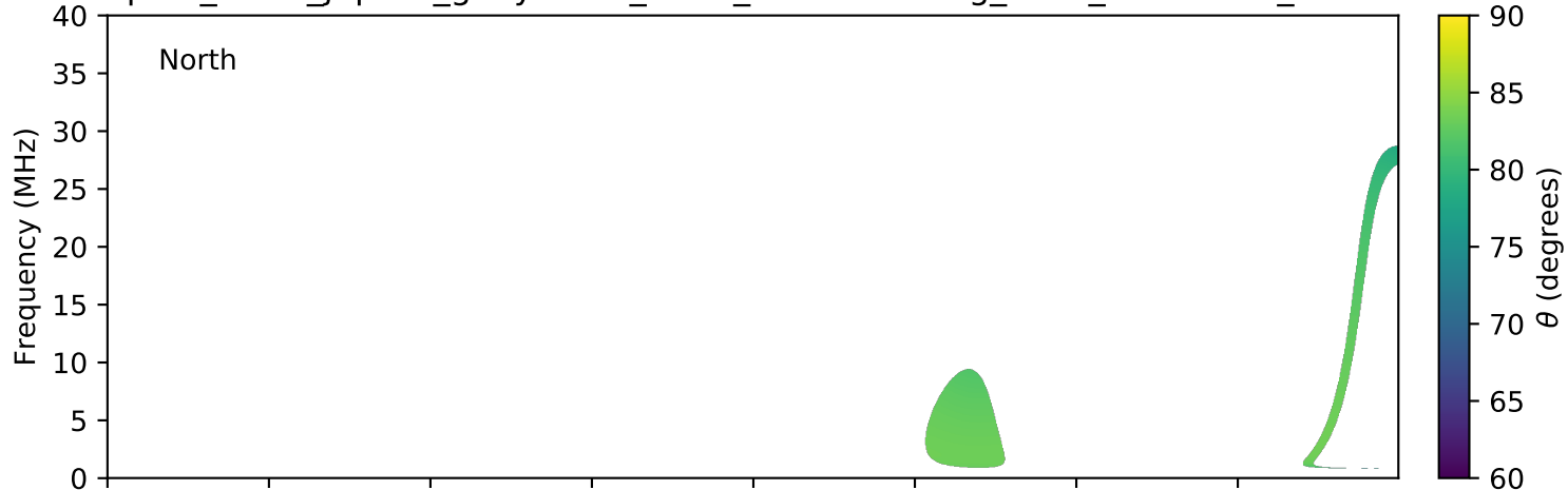
expres_earth_jupiter_ganymede_isaac_lossc-wid1deg_3kev_20160222_v01.cdf
