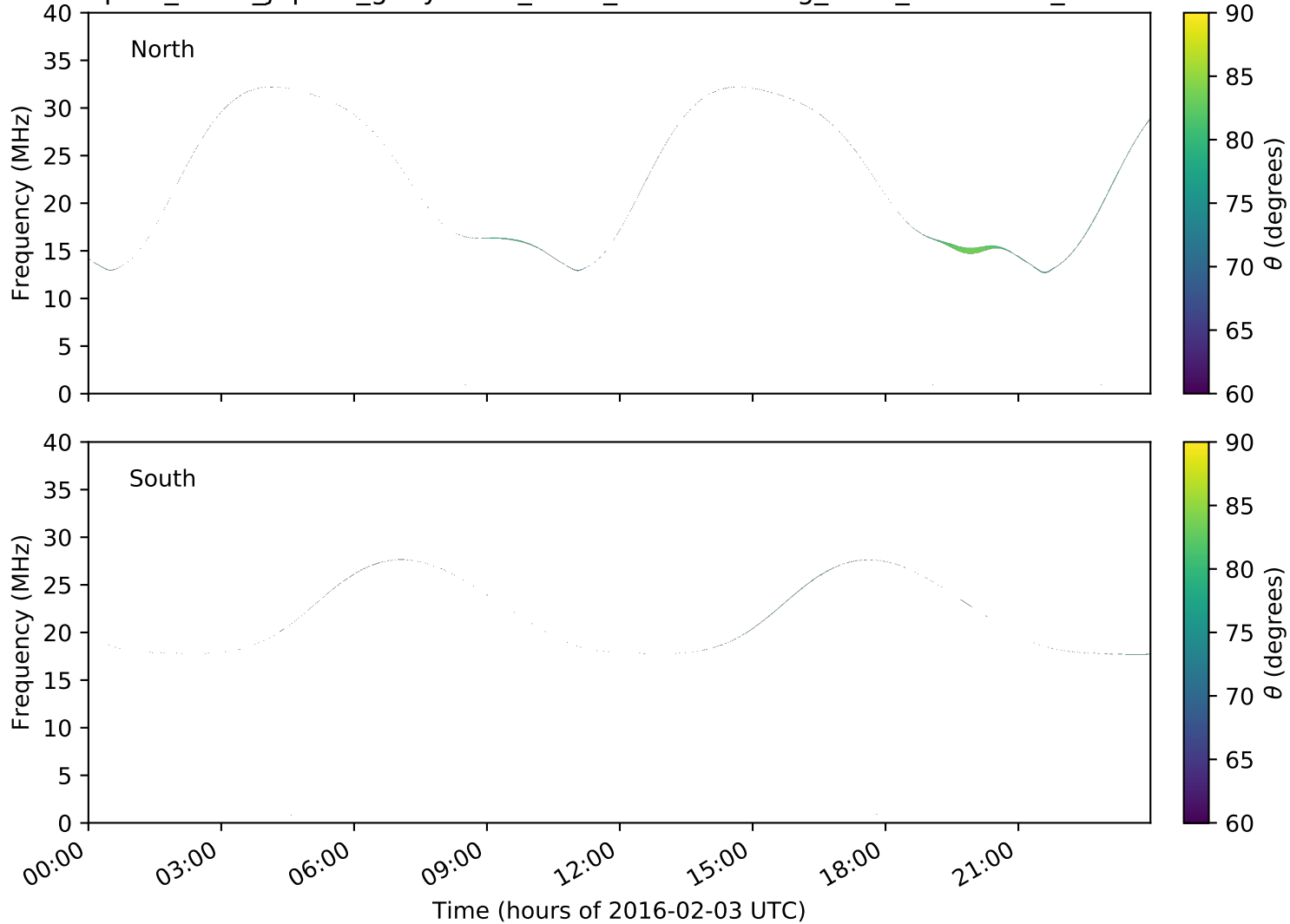
expres_earth_jupiter_ganymede_isaac_lossc-wid1deg_1kev_20160203_v01.cdf
