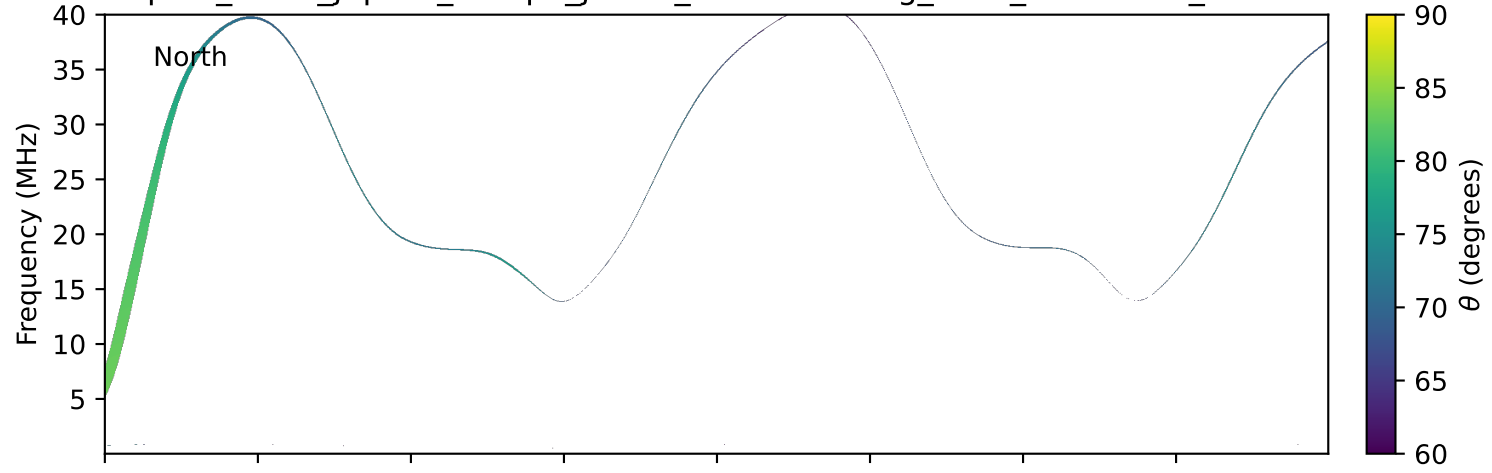
expres_earth_jupiter_europa_jrm33_lossc-wid1deg_3kev_20160208_v11.cdf
