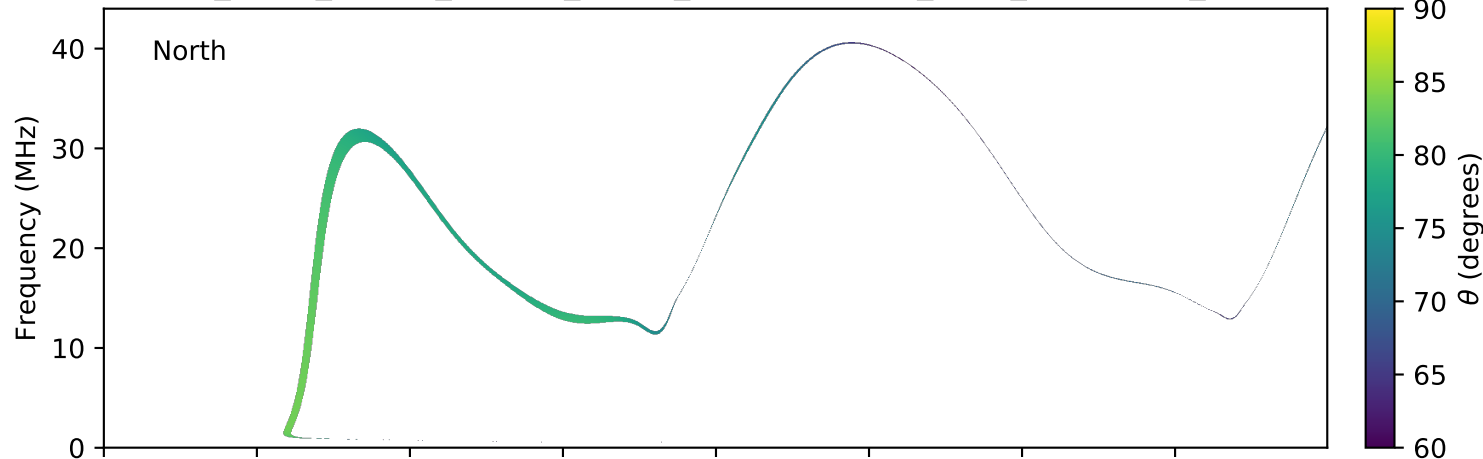
expres_earth_jupiter_europa_jrm09_lossc-wid1deg_3kev_20160229_v01.cdf
