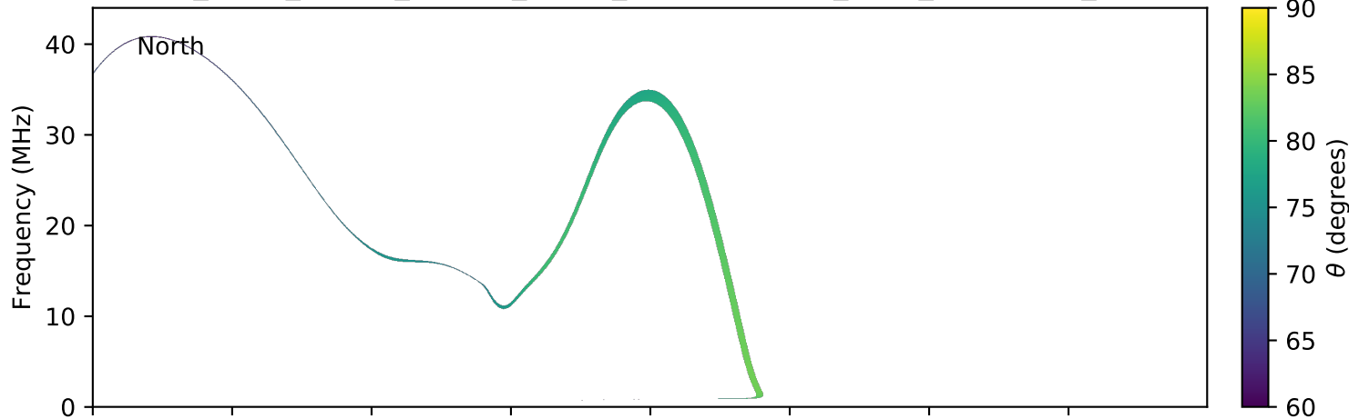
expres_earth_jupiter_europa_jrm09_lossc-wid1deg_3kev_20160223_v01.cdf
