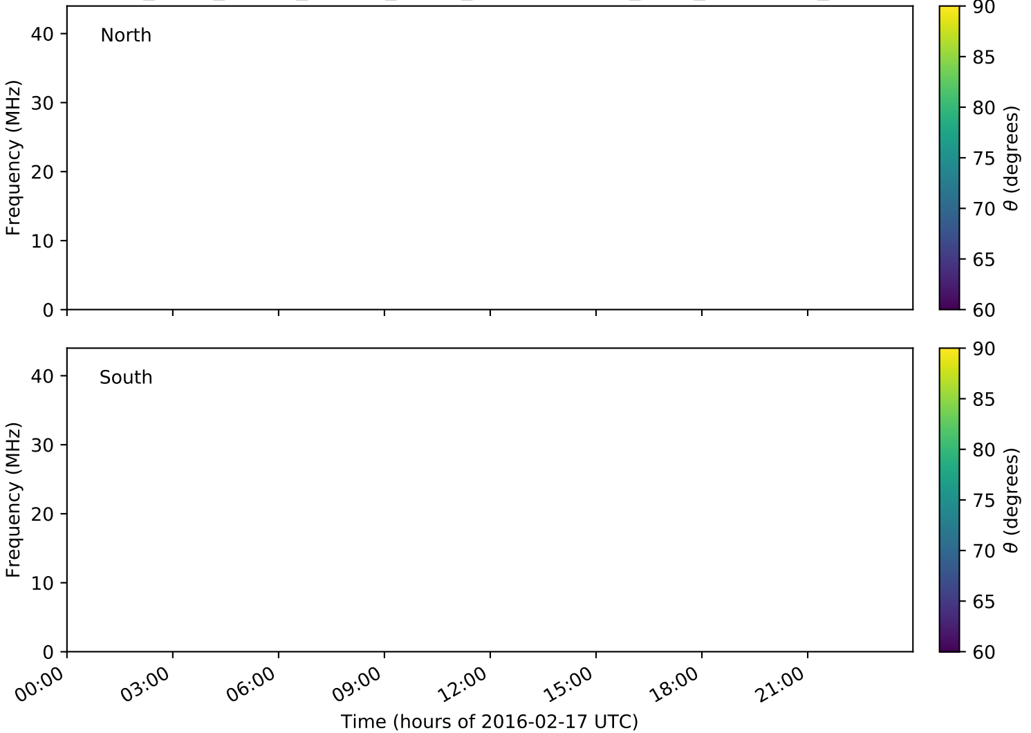
expres_earth_jupiter_europa_jrm09_lossc-wid1deg_3kev_20160217_v01.cdf
