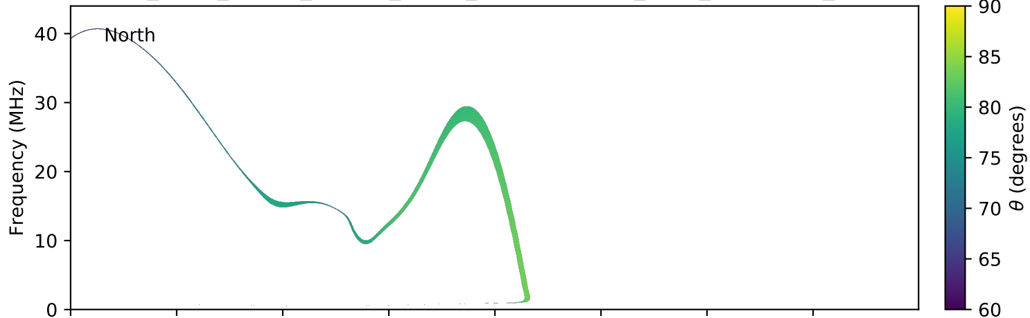
expres_earth_jupiter_europa_jrm09_lossc-wid1deg_3kev_20160216_v01.cdf
