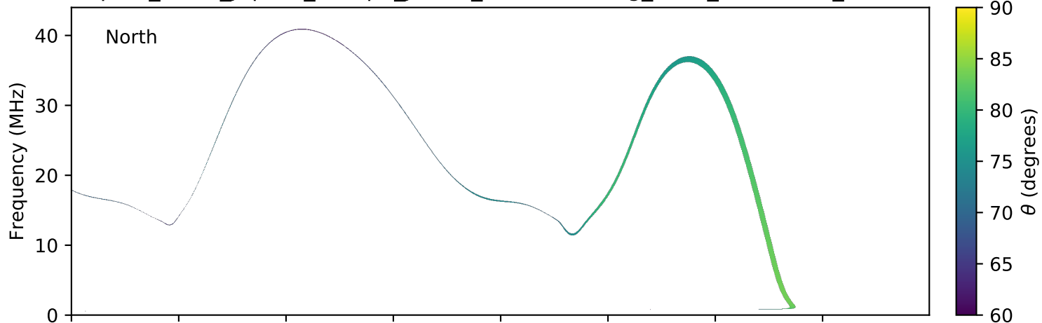
expres_earth_jupiter_europa_jrm09_lossc-wid1deg_3kev_20160205_v01.cdf
