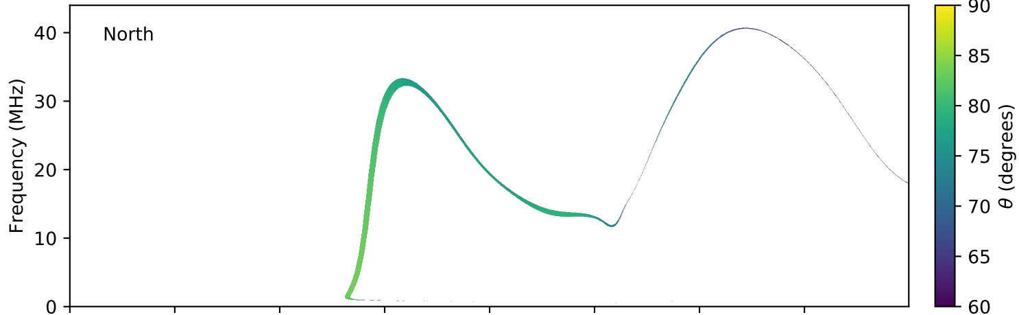
expres_earth_jupiter_europa_jrm09_lossc-wid1deg_3kev_20160204_v01.cdf
