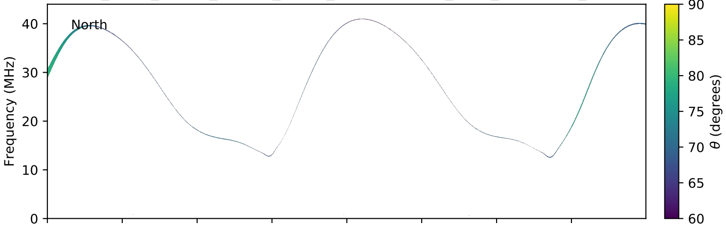
expres_earth_jupiter_europa_jrm09_lossc-wid1deg_3kev_20160201_v01.cdf
