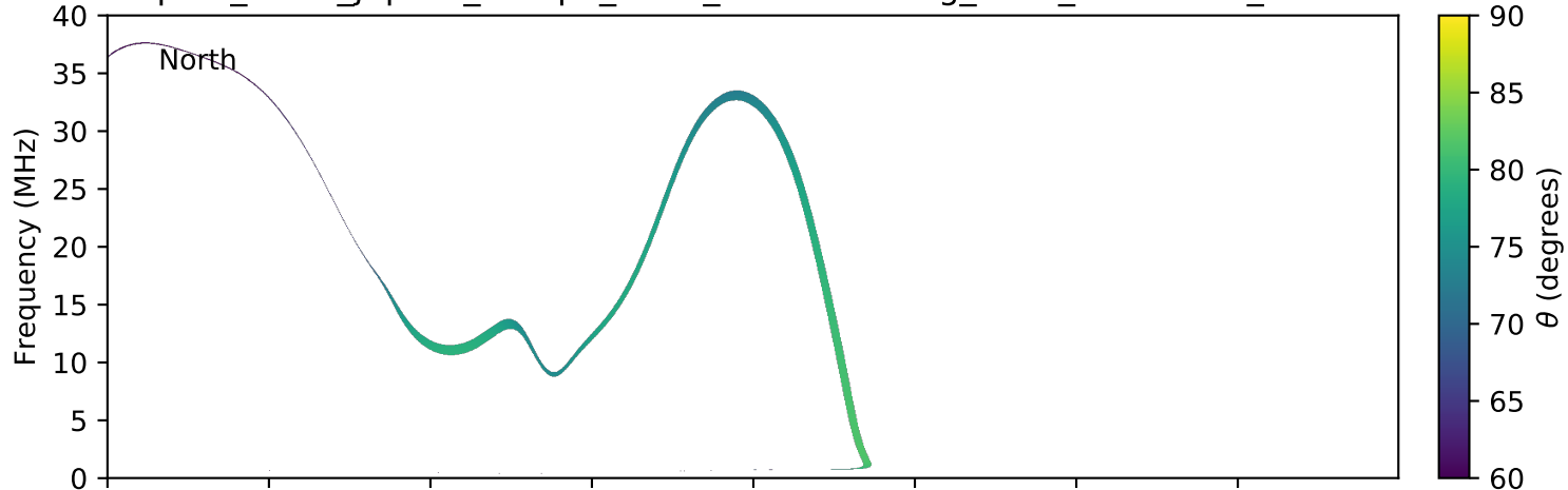
expres_earth_jupiter_europa_isaac_lossc-wid1deg_5kev_20160223_v01.cdf
