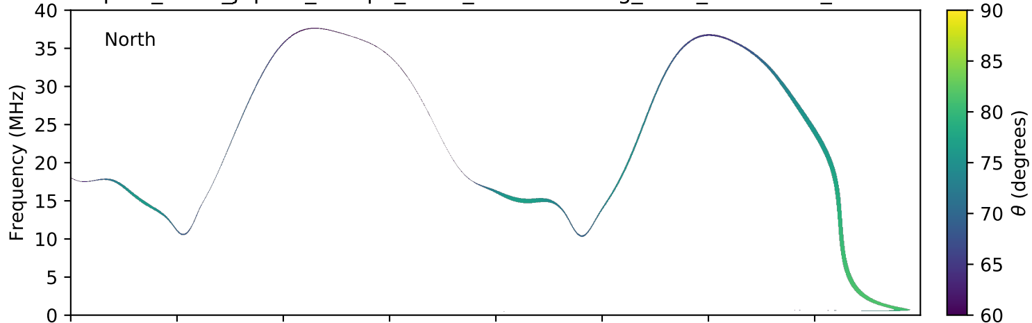
expres_earth_jupiter_europa_isaac_lossc-wid1deg_5kev_20160219_v01.cdf
