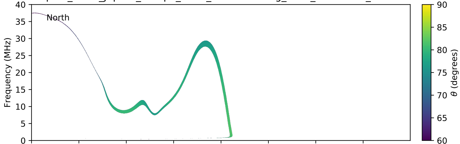
expres_earth_jupiter_europa_isaac_lossc-wid1deg_5kev_20160216_v01.cdf
