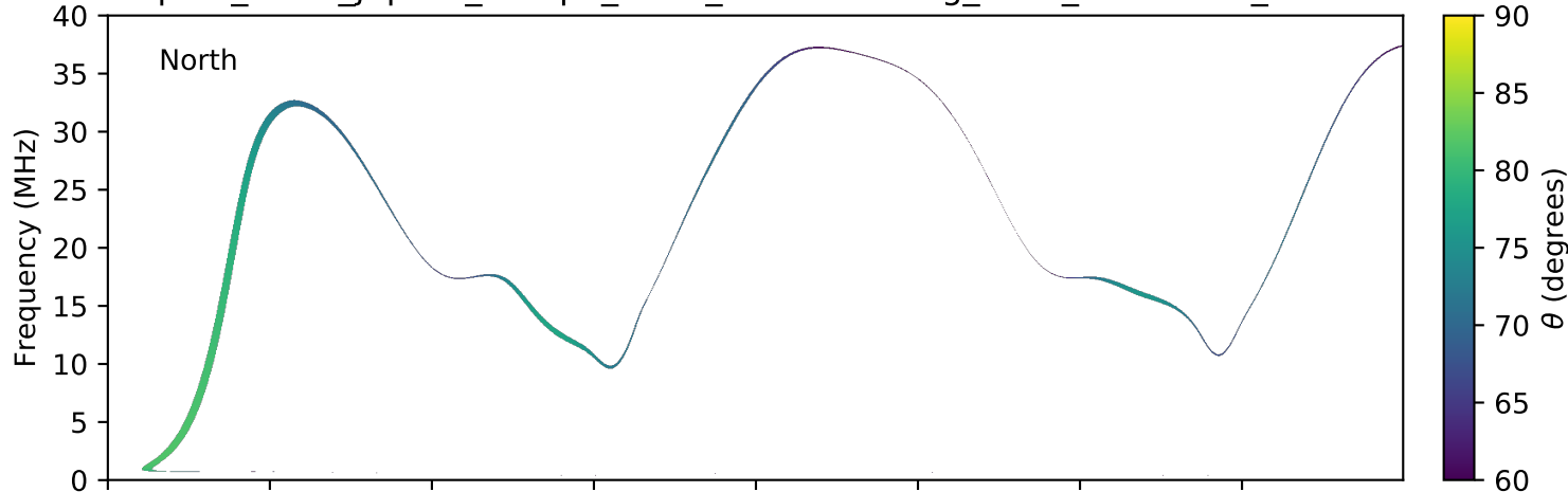
expres_earth_jupiter_europa_isaac_lossc-wid1deg_5kev_20160215_v01.cdf
