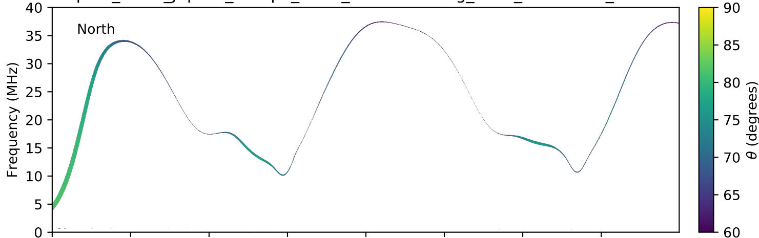
expres_earth_jupiter_europa_isaac_lossc-wid1deg_5kev_20160208_v01.cdf
