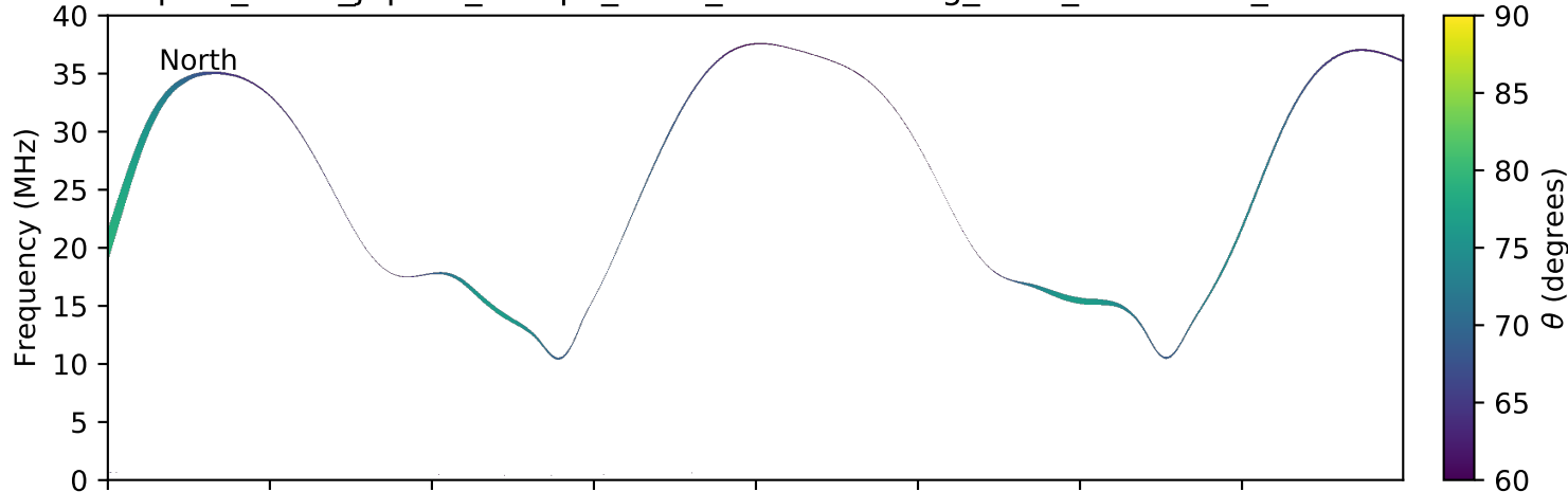
expres_earth_jupiter_europa_isaac_lossc-wid1deg_5kev_20160201_v01.cdf
