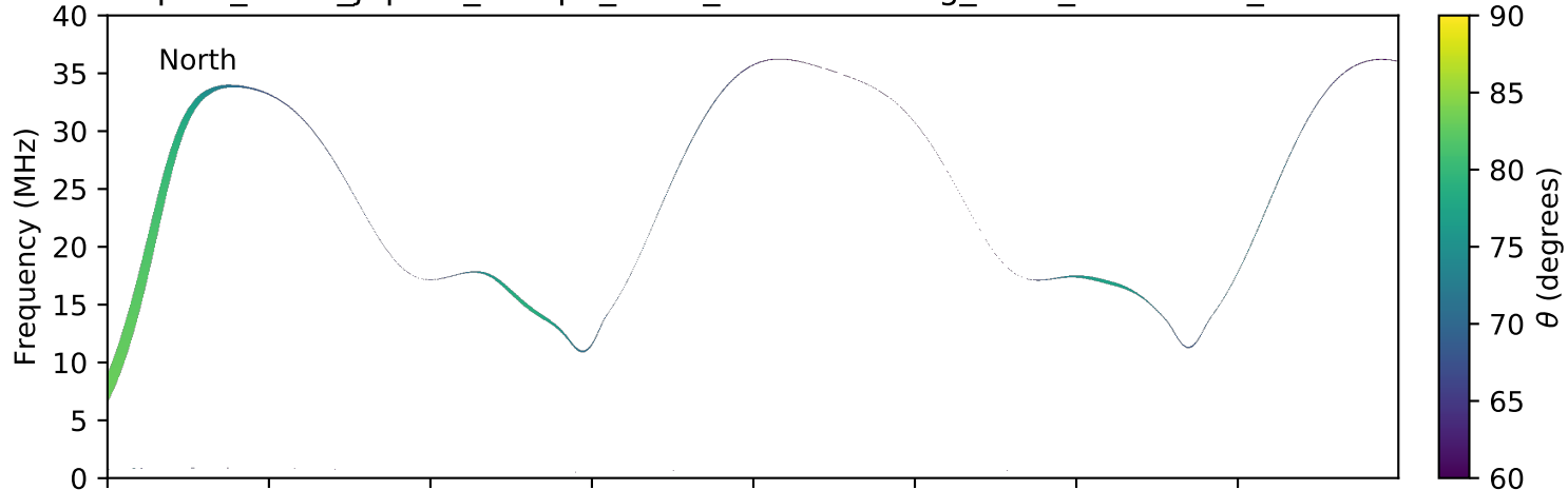
expres_earth_jupiter_europa_isaac_lossc-wid1deg_3kev_20160208_v01.cdf
